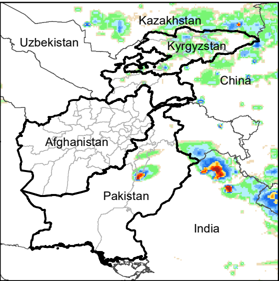
Daily Rainfall estimate for 8 Aug., 2009
