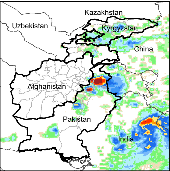
Daily Rainfall estimate for 19 Aug., 2009
