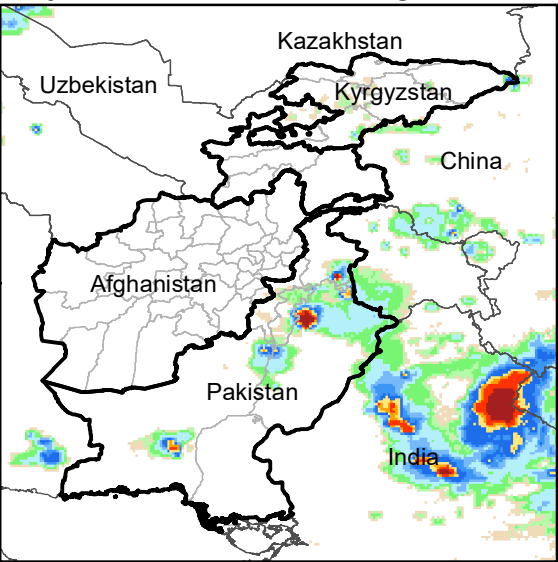
Daily Rainfall estimate for 20 Aug., 2009
