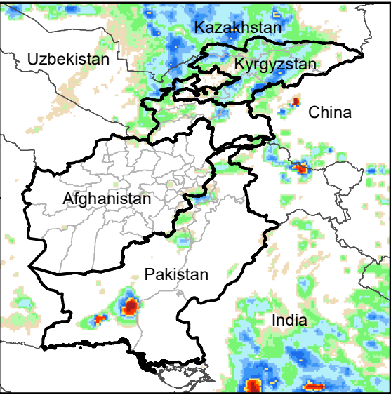
Daily Rainfall estimate for 25 Aug., 2009
