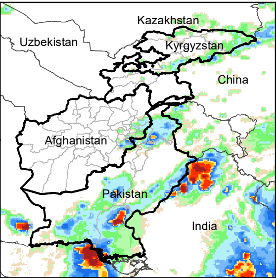
Daily Rainfall estimate for 3 Sep., 2009
