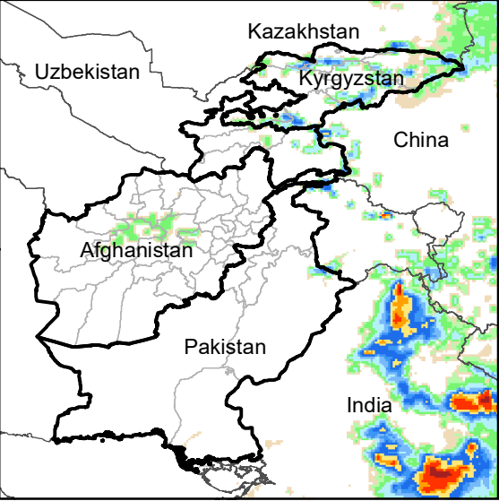
Daily Rainfall estimate for 10 Sep., 2009
