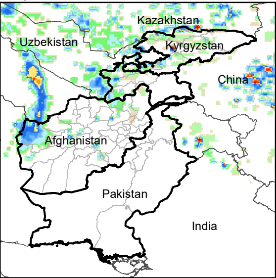
Daily Rainfall estimate for 23 Nov., 2009
