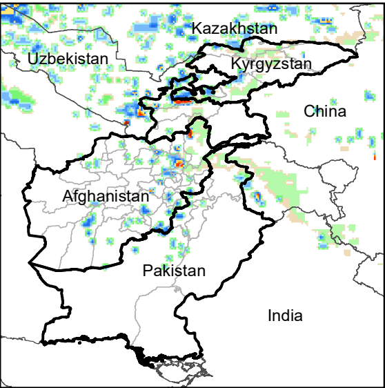
Daily Rainfall estimate for 22 Nov., 2009
