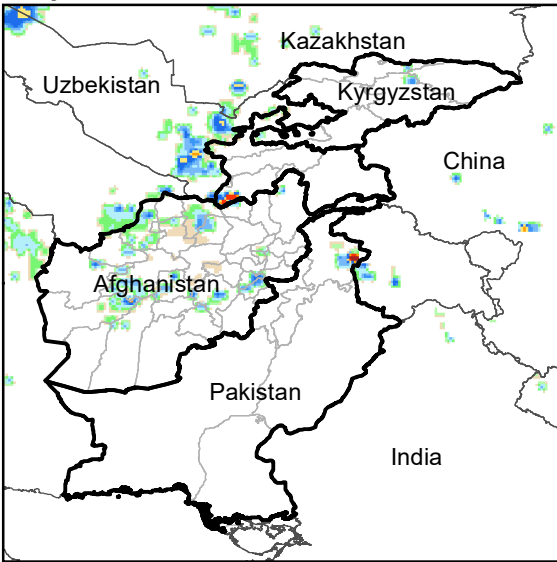
Daily Rainfall estimate for 6 Dec., 2009
