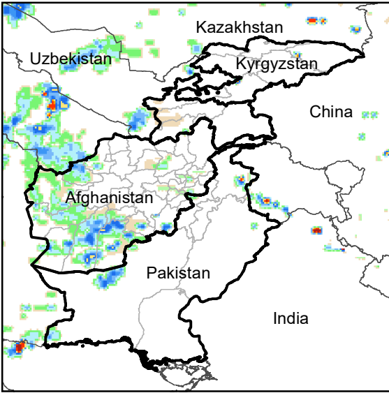
Daily Rainfall estimate for 19 Dec., 2009
