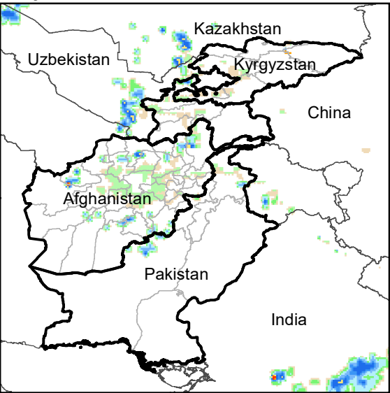
Daily Rainfall estimate for 20 Dec., 2009
