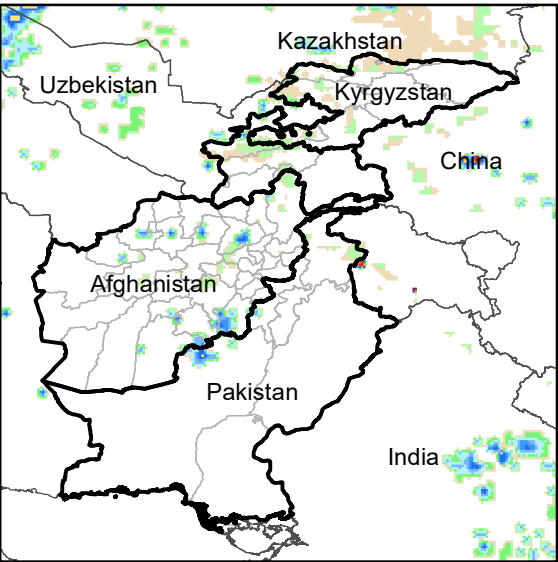
Daily Rainfall estimate for 2 Jan., 2010
