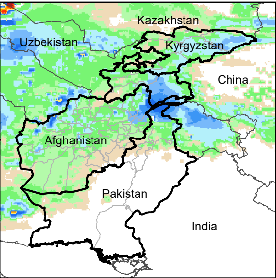
Daily Rainfall estimate for 8 Feb., 2010
