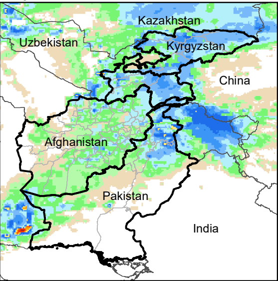
Daily Rainfall estimate for 9 Feb., 2010
