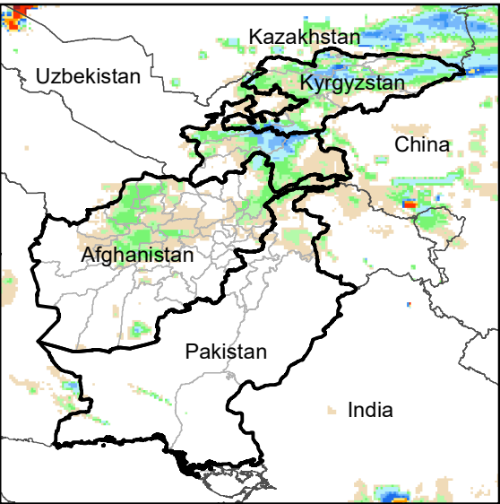
Daily Rainfall estimate for 7 Feb., 2010
