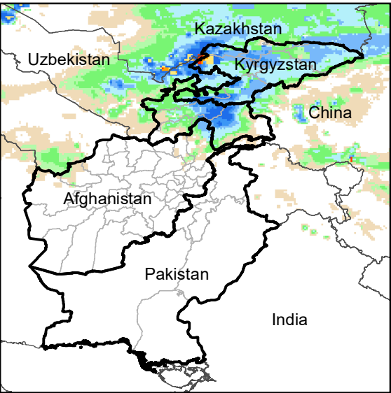
Daily Rainfall estimate for 22 Feb., 2010
