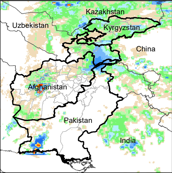
Daily Rainfall estimate for 25 Feb., 2010
