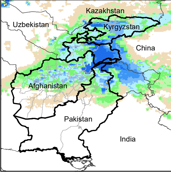
Daily Rainfall estimate for 26 Feb., 2010
