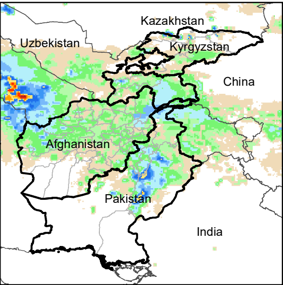
Daily Rainfall estimate for 6 Mar., 2010
