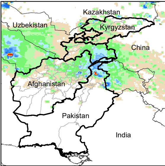
Daily Rainfall estimate for 1 Apr., 2010
