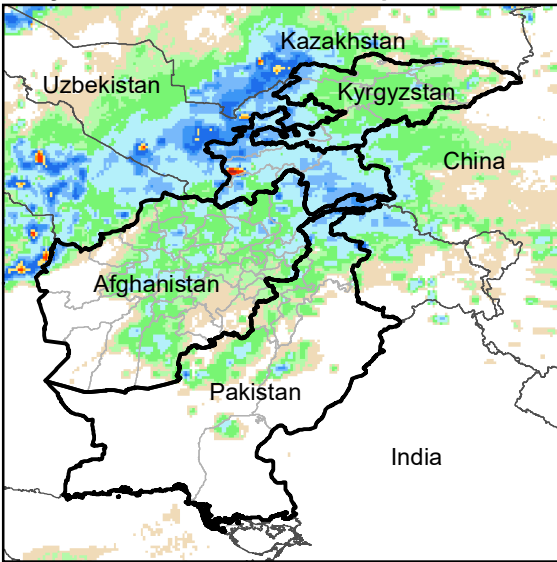
Daily Rainfall estimate for 14 Apr., 2010
