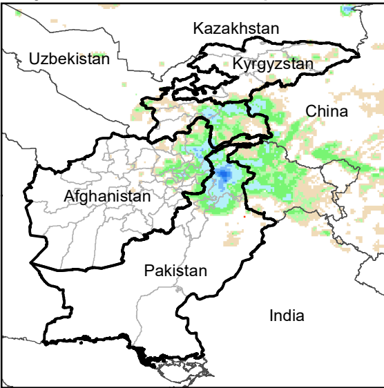
Daily Rainfall estimate for 25 Apr., 2010
