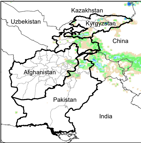
Daily Rainfall estimate for 26 Apr., 2010
