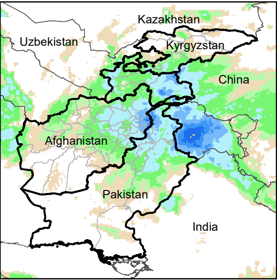
Daily Rainfall estimate for 5 May., 2010
