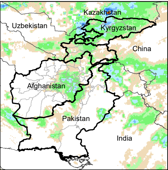
Daily Rainfall estimate for 4 May., 2010
