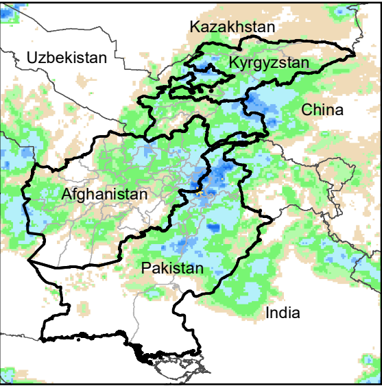
Daily Rainfall estimate for 6 May., 2010
