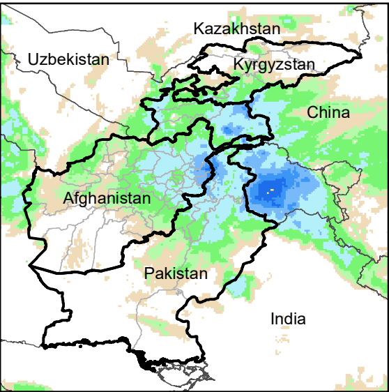
Daily Rainfall estimate for 8 May., 2010
