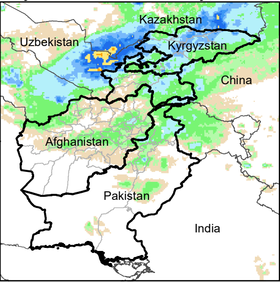
Daily Rainfall estimate for 22 May., 2010
