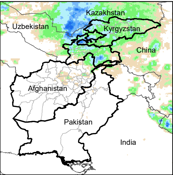
Daily Rainfall estimate for 29 May., 2010
