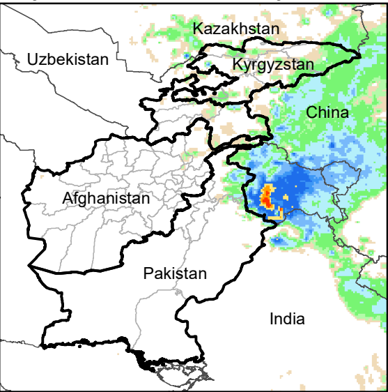
Daily Rainfall estimate for 31 May., 2010
