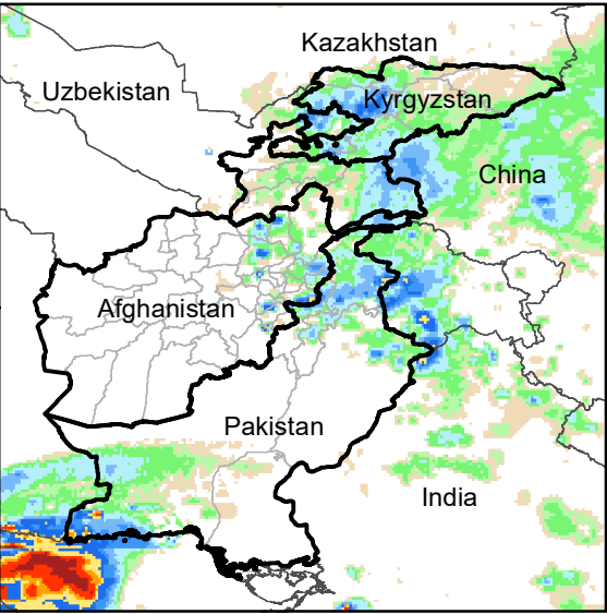
Daily Rainfall estimate for 4 Jun., 2010
