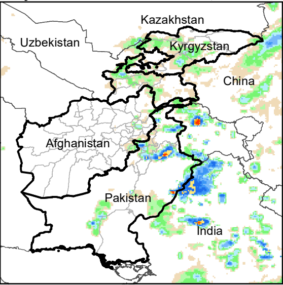
Daily Rainfall estimate for 25 Jun., 2010
