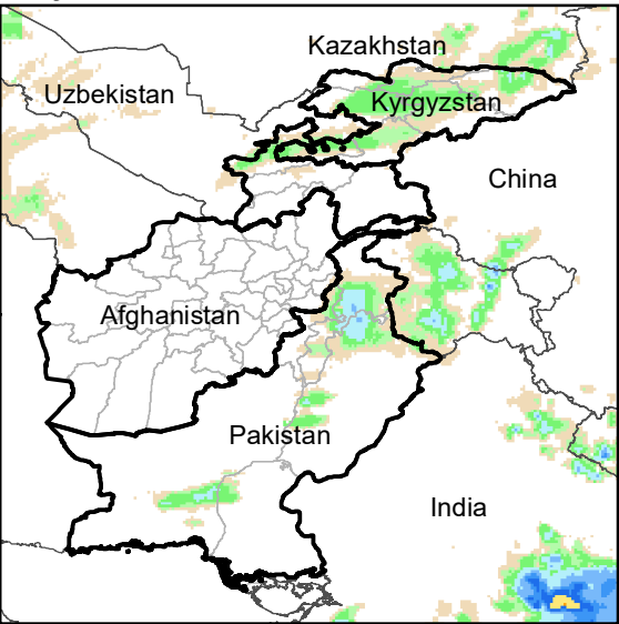
Daily Rainfall estimate for 26 Jun., 2010
