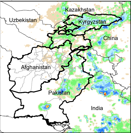
Daily Rainfall estimate for 27 Jun., 2010
