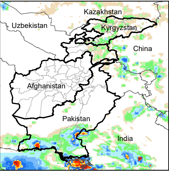
Daily Rainfall estimate for 8 Jul., 2010
