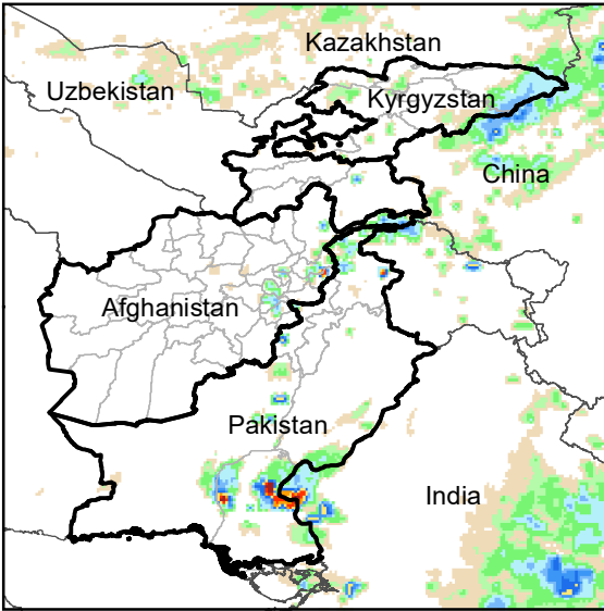
Daily Rainfall estimate for 14 Jul., 2010
