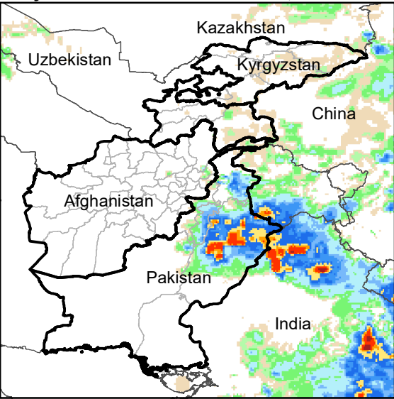
Daily Rainfall estimate for 12 Jul., 2010
