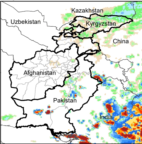
Daily Rainfall estimate for 13 Jul., 2010
