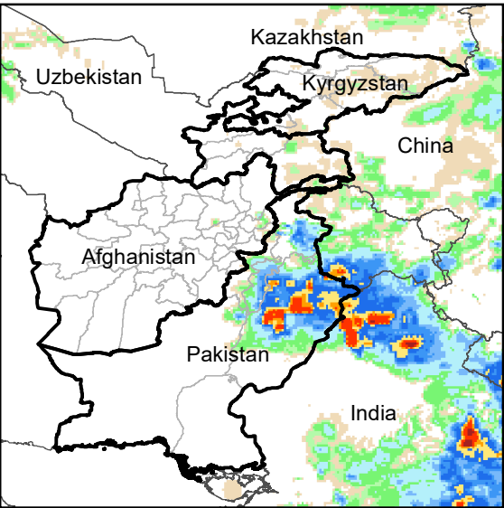
Daily Rainfall estimate for 15 Jul., 2010
