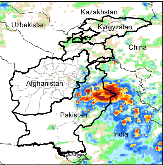
Daily Rainfall estimate for 23 Jul., 2010
