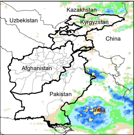
Daily Rainfall estimate for 21 Jul., 2010
