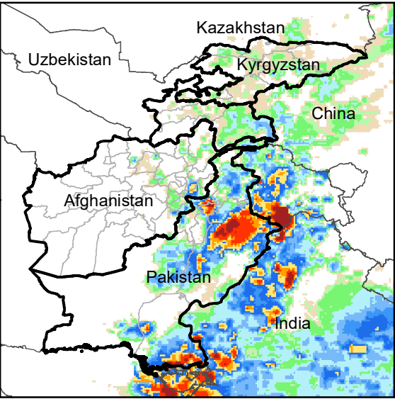
Daily Rainfall estimate for 22 Jul., 2010
