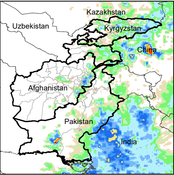
Daily Rainfall estimate for 31 Jul., 2010
