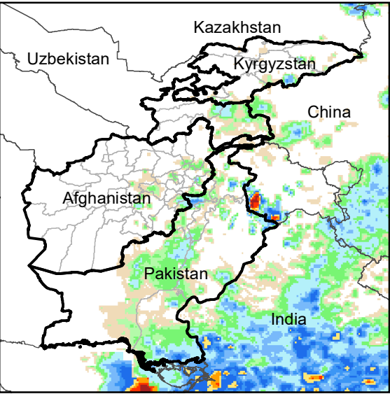
Daily Rainfall estimate for 1 Aug., 2010
