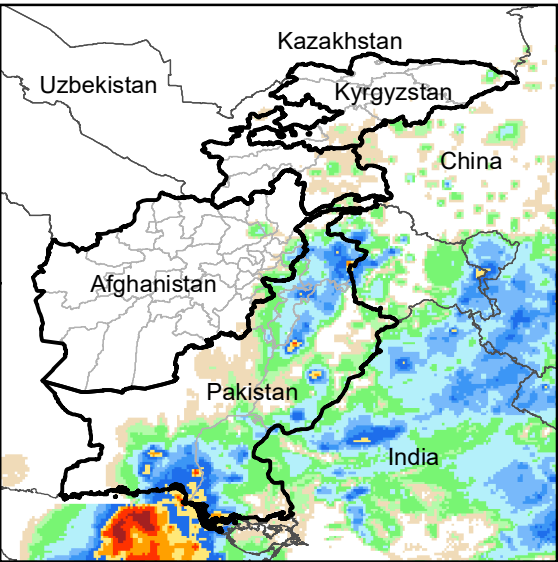
Daily Rainfall estimate for 30 Jul., 2010
