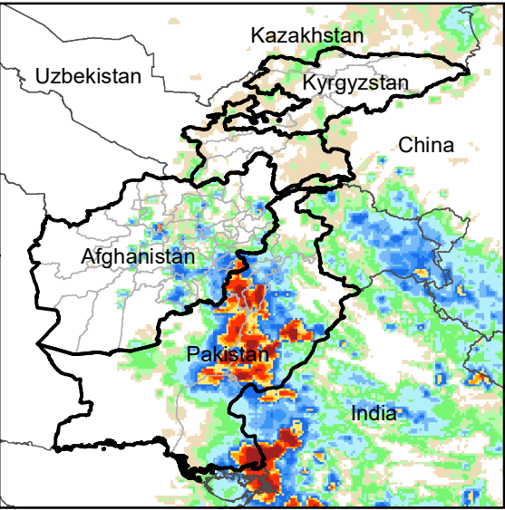
Daily Rainfall estimate for 4 Aug., 2010
