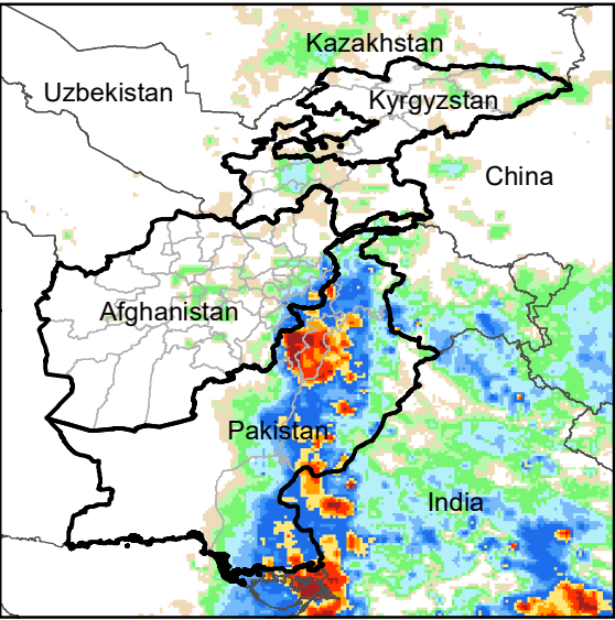
Daily Rainfall estimate for 3 Aug., 2010
