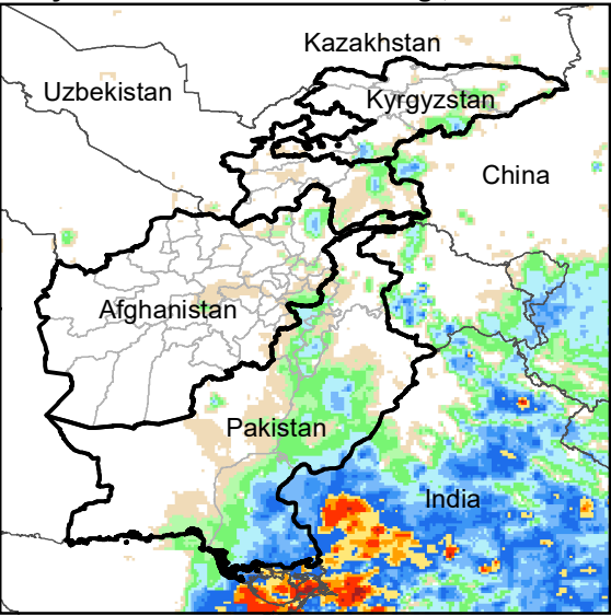
Daily Rainfall estimate for 2 Aug., 2010
