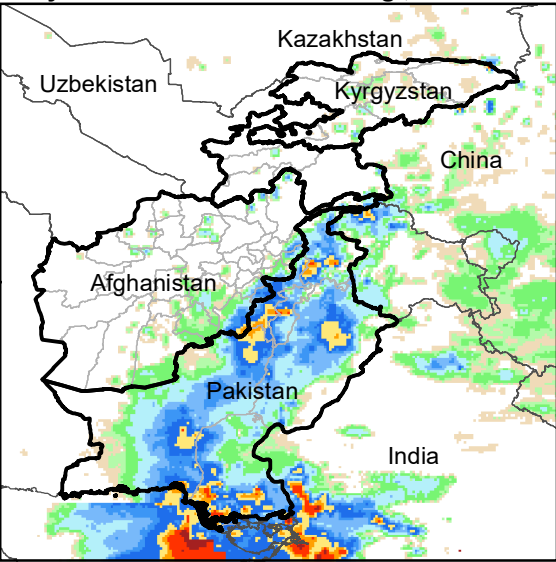
Daily Rainfall estimate for 8 Aug., 2010
