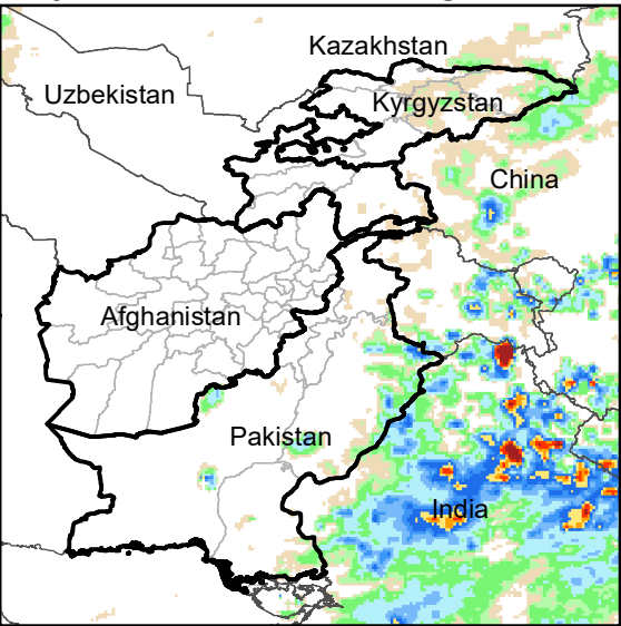
Daily Rainfall estimate for 24 Aug., 2010
