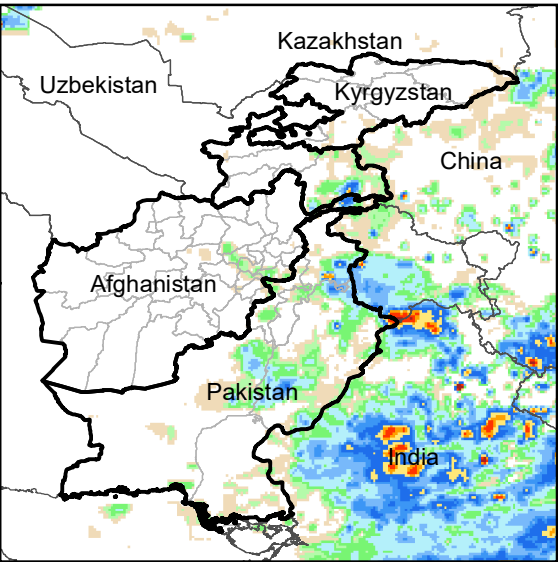
Daily Rainfall estimate for 23 Aug., 2010
