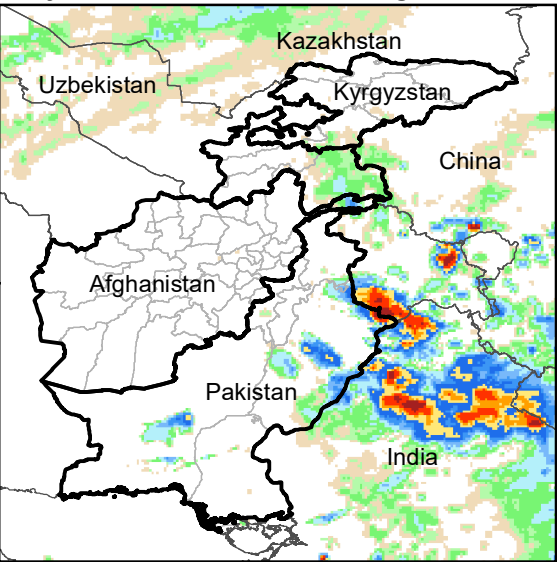
Daily Rainfall estimate for 25 Aug., 2010
