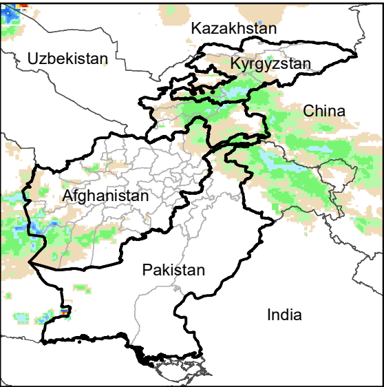
Daily Rainfall estimate for 31 Jan., 2011
