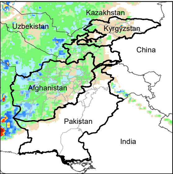
Daily Rainfall estimate for 5 Feb., 2011
