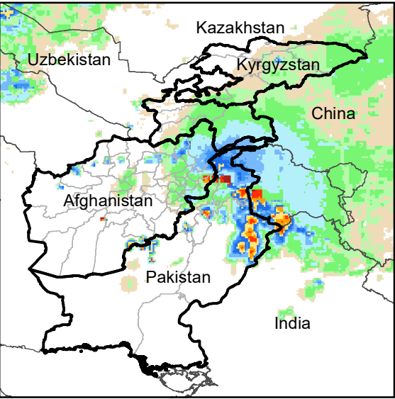
Daily Rainfall estimate for 7 Feb., 2011
