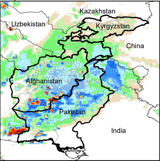
Daily Rainfall estimate for 12 Feb., 2011
