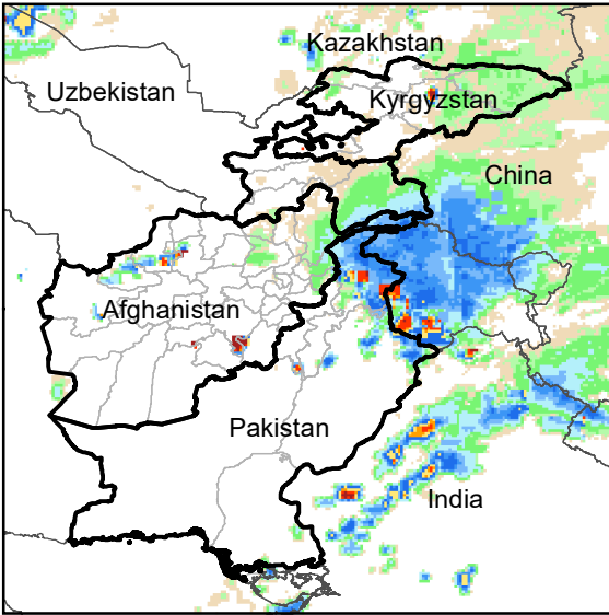
Daily Rainfall estimate for 14 Feb., 2011
