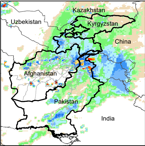
Daily Rainfall estimate for 13 Feb., 2011
