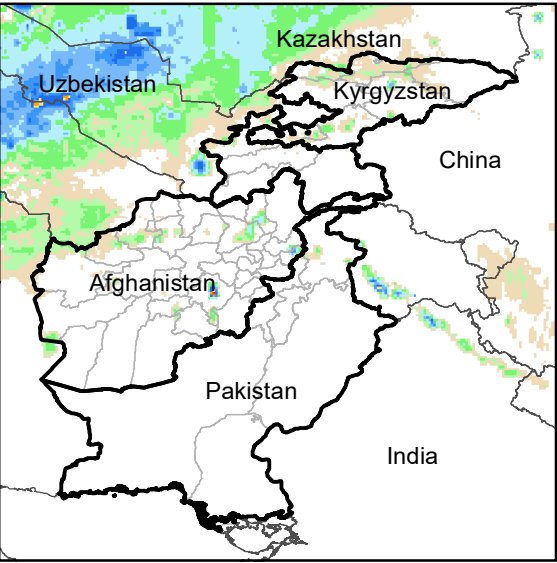
Daily Rainfall estimate for 14 Mar., 2011
