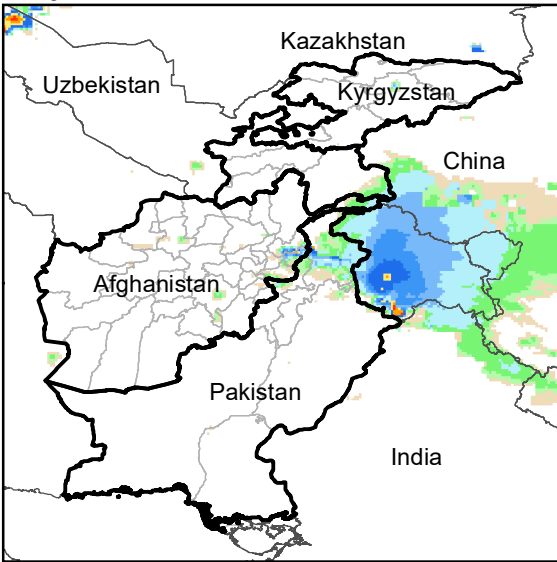
Daily Rainfall estimate for 22 Mar., 2011
