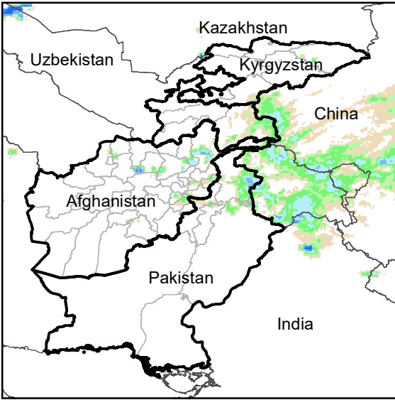
Daily Rainfall estimate for 29 Mar., 2011
