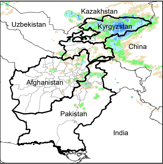
Daily Rainfall estimate for 31 Mar., 2011
