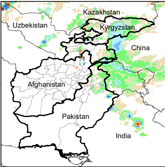
Daily Rainfall estimate for 5 Apr., 2011
