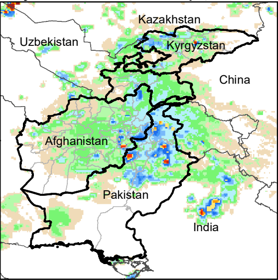
Daily Rainfall estimate for 10 Apr., 2011
