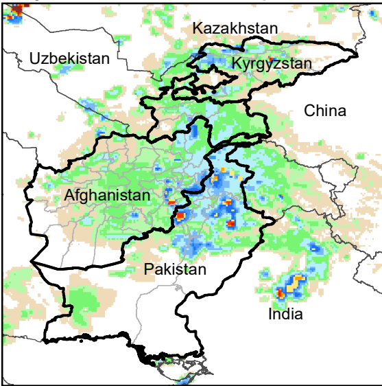
Daily Rainfall estimate for 13 Apr., 2011
