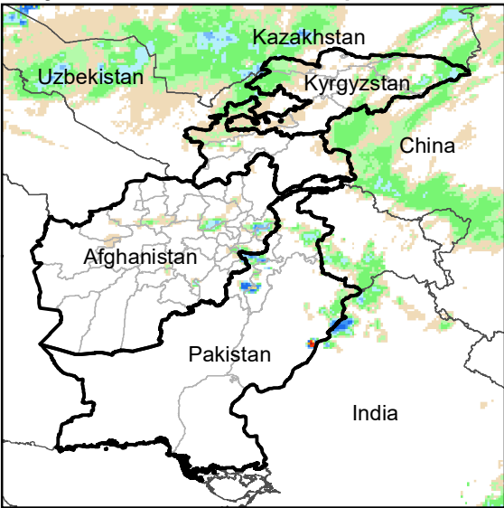
Daily Rainfall estimate for 22 Apr., 2011
