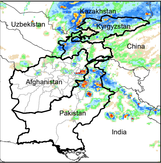
Daily Rainfall estimate for 6 May., 2011
