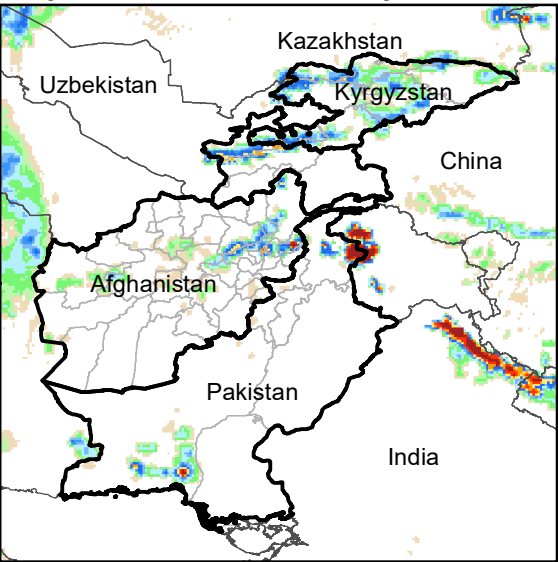
Daily Rainfall estimate for 5 May., 2011
