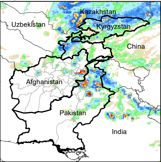
Daily Rainfall estimate for 9 May., 2011
