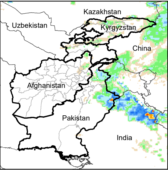
Daily Rainfall estimate for 1 Jun., 2011
