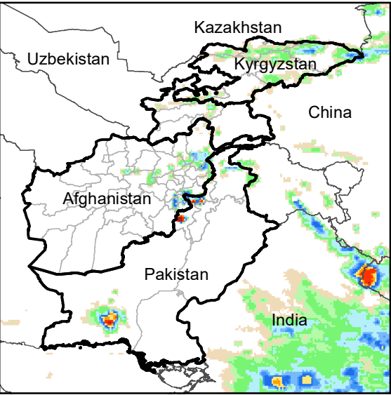
Daily Rainfall estimate for 5 Jul., 2011
