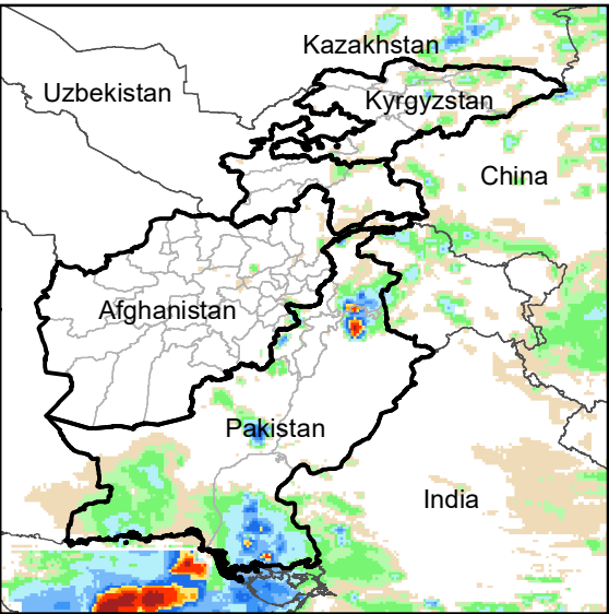
Daily Rainfall estimate for 29 Jul., 2011
