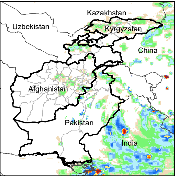
Daily Rainfall estimate for 3 Aug., 2011
