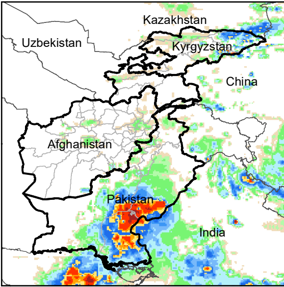
Daily Rainfall estimate for 31 Aug., 2011
