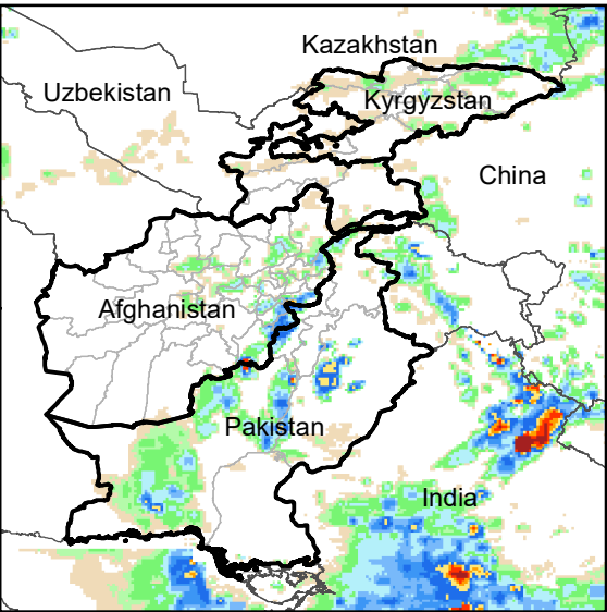
Daily Rainfall estimate for 29 Aug., 2011
