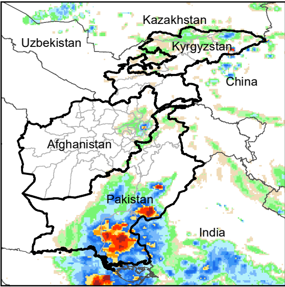
Daily Rainfall estimate for 30 Aug., 2011
